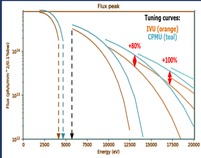
CPMU vs IVU: 2x more flux
