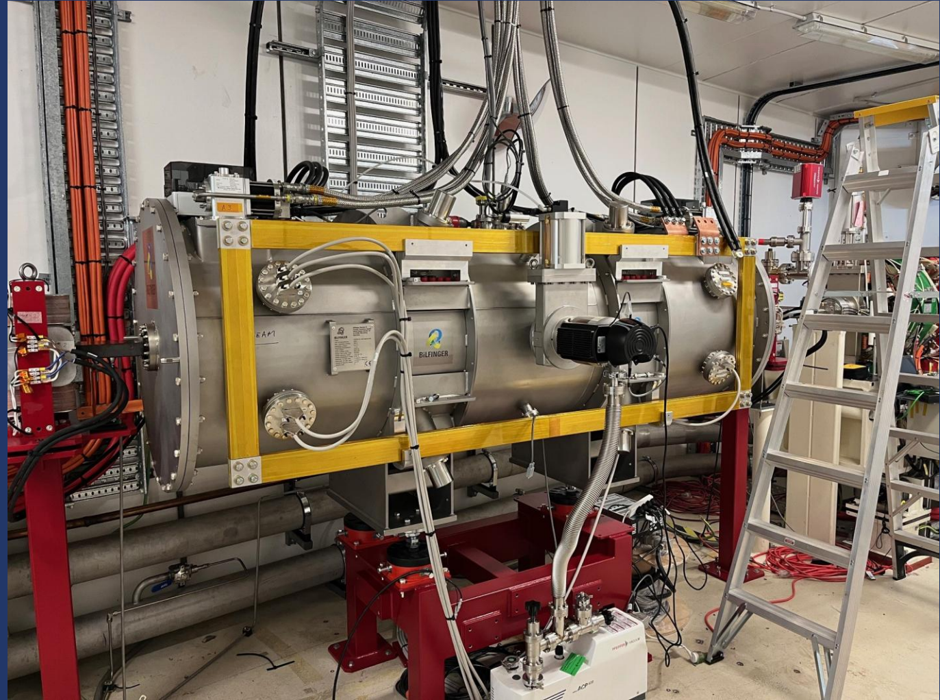
ADS SCMPW in the Storage Ring (sector 10 ID) Commissioning begins in February 2026
