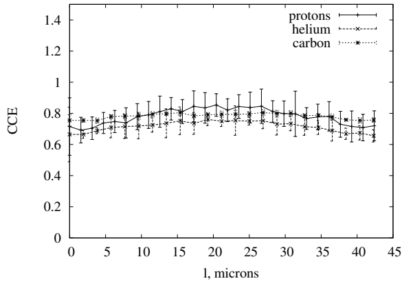
Fig. 13. Charge collection efficiency profiles for 10\ \mu\text{m} device at bias of 10\ \text{V} . l is distance along diagonal of figure 3
