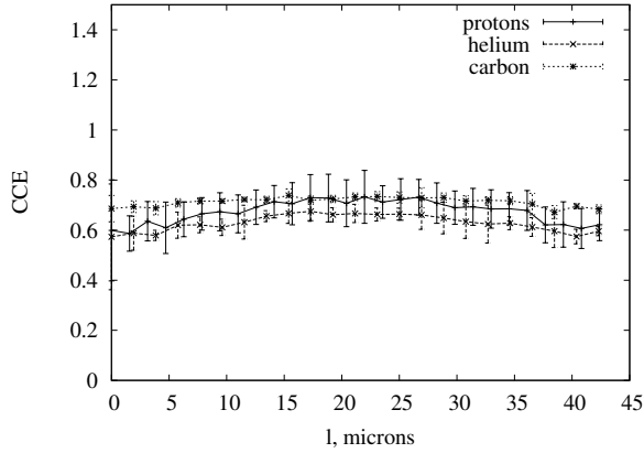
Fig. 12. Charge collection efficiency profiles for 10\ \mu\text{m} device at bias of 0\ \text{V} . l is distance along diagonal of figure 3
