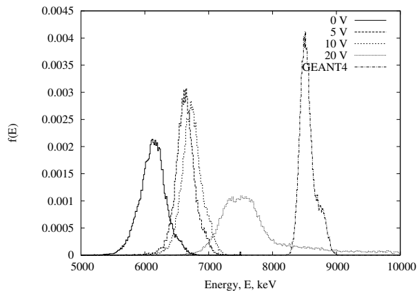
Fig. 9. Simulated and experimental IBIC spectra for 25 MeV carbon scan of 10 μm device at given bias.
