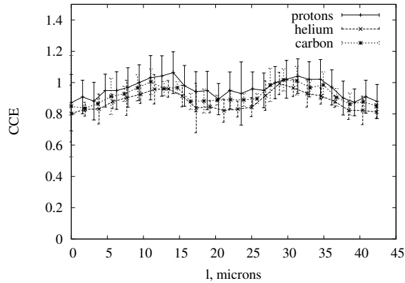
Fig. 17. Charge collection efficiency profiles for 5\ \mu\text{m} device at bias of 20\ \text{V} . l is distance along diagonal of figure 3
