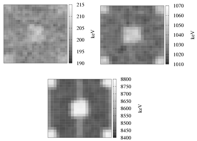
Fig. 11. Simulated IBIC image for 10 μm device with 3 MeV protons (top left), 9 MeV helium (top right), and 25 MeV carbon (bottom).
