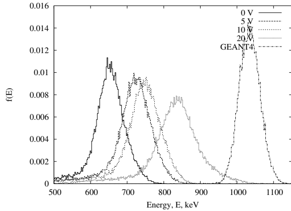
Fig. 7. Simulated and experimental IBIC spectra for 9 MeV helium scan of 10 μm device.
