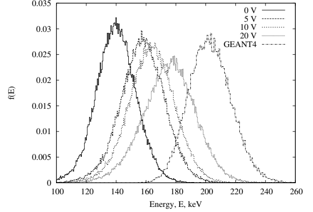
Fig. 5. Simulated and experimental IBIC spectra for 3 MeV proton scan of 10 \mu m device.
