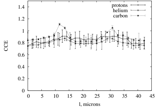
Fig. 14. Charge collection efficiency profiles for 10\ \mu\text{m} device at bias of 20\ \text{V} . l is distance along diagonal of figure 3
