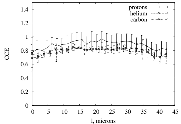
Fig. 16. Charge collection efficiency profiles for 5\ \mu\text{m} device at bias of 10\ \text{V} . l is distance along diagonal of figure 3
