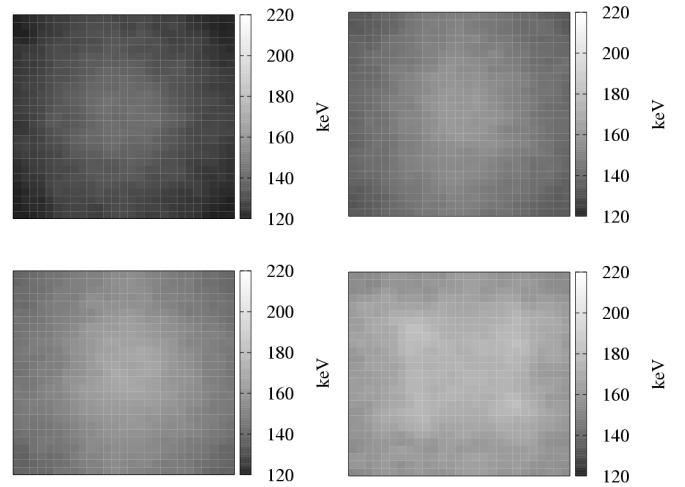
Fig. 6. Experimental IBIC median energy images for 3 MeV proton scan of 10 \mu m device at bias of 0 V (top left) and 5 V (top right), 10 V (bottom left), 20 V (bottom right).
