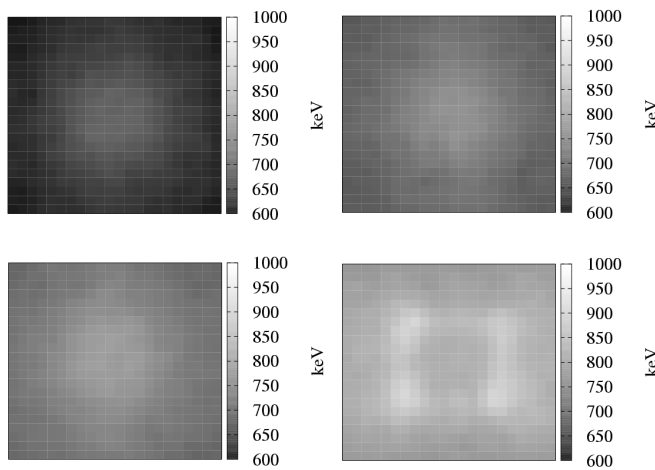
Fig. 8. Experimental IBIC median energy image for 9 MeV helium scan of 10 μm device at bias of 0 V (top left) and 5 V (top right), 10 V (bottom left), 20 V (bottom right).
