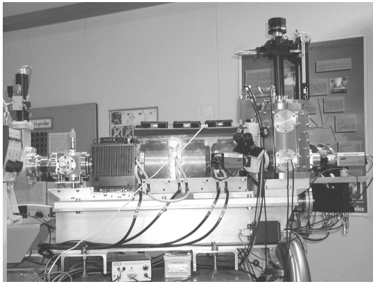
Fig. 2. ANSTO heavy ion microprobe end station.
