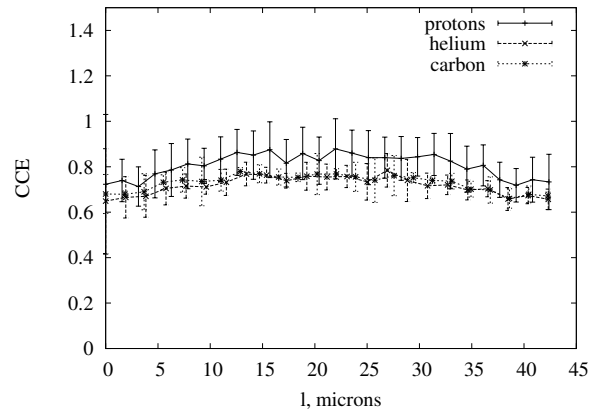
Fig. 15. Charge collection efficiency profiles for 5\ \mu\text{m} device at bias of 0\ \text{V} . l is distance along diagonal of figure 3
