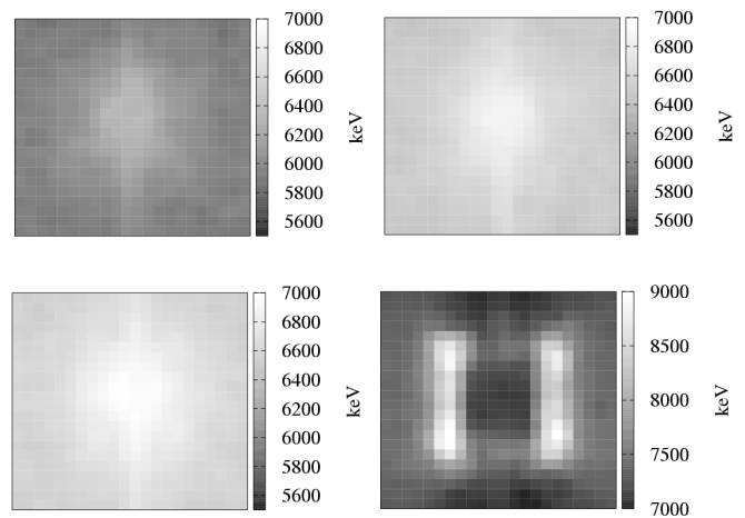
Fig. 10. Experimental IBIC median energy image for 25 MeV carbon scan of 10 μm device at bias of 0 V (top left) and 5 V (top right), 10 V (bottom left), 20 V (bottom right).
